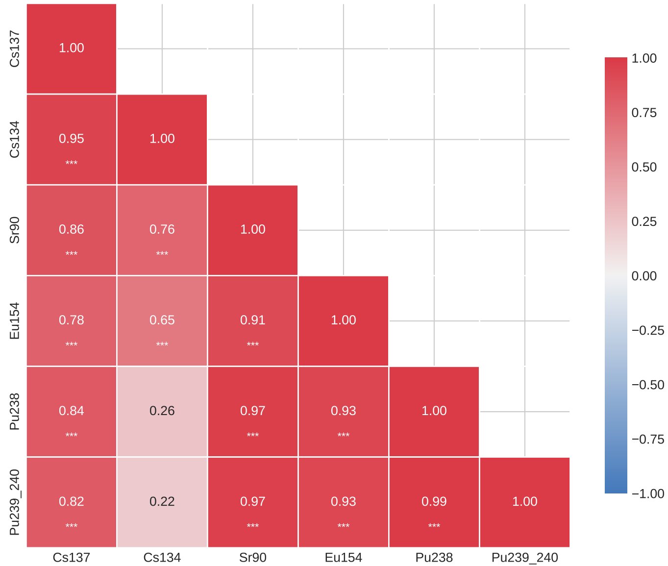
Cross-Radionuclide Correlation (* p<.05 ** p<.01 *** p<.001)
