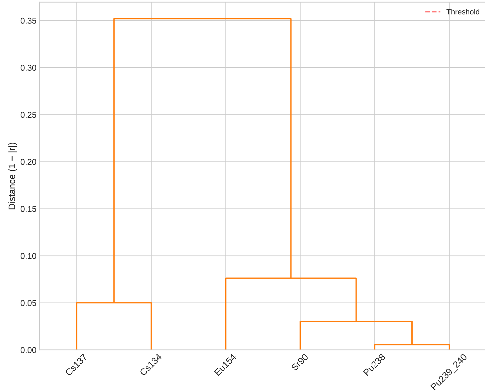
Hierarchical Clustering of Radionuclides
